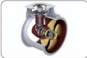
THRUSTER
